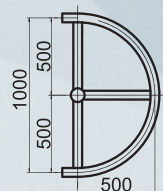
Wspornik K4-1.0-1.0 (M1ak, M2ak)
